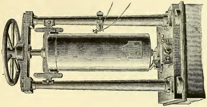
Borland's Dead-Weight Pressure Gauge.
